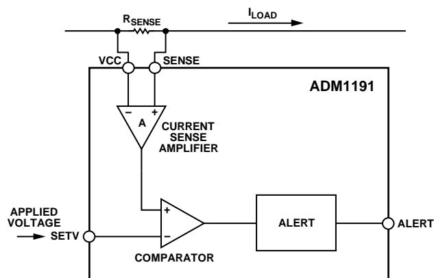
Figure 26. SETV Operation
